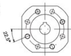
RV150,185
